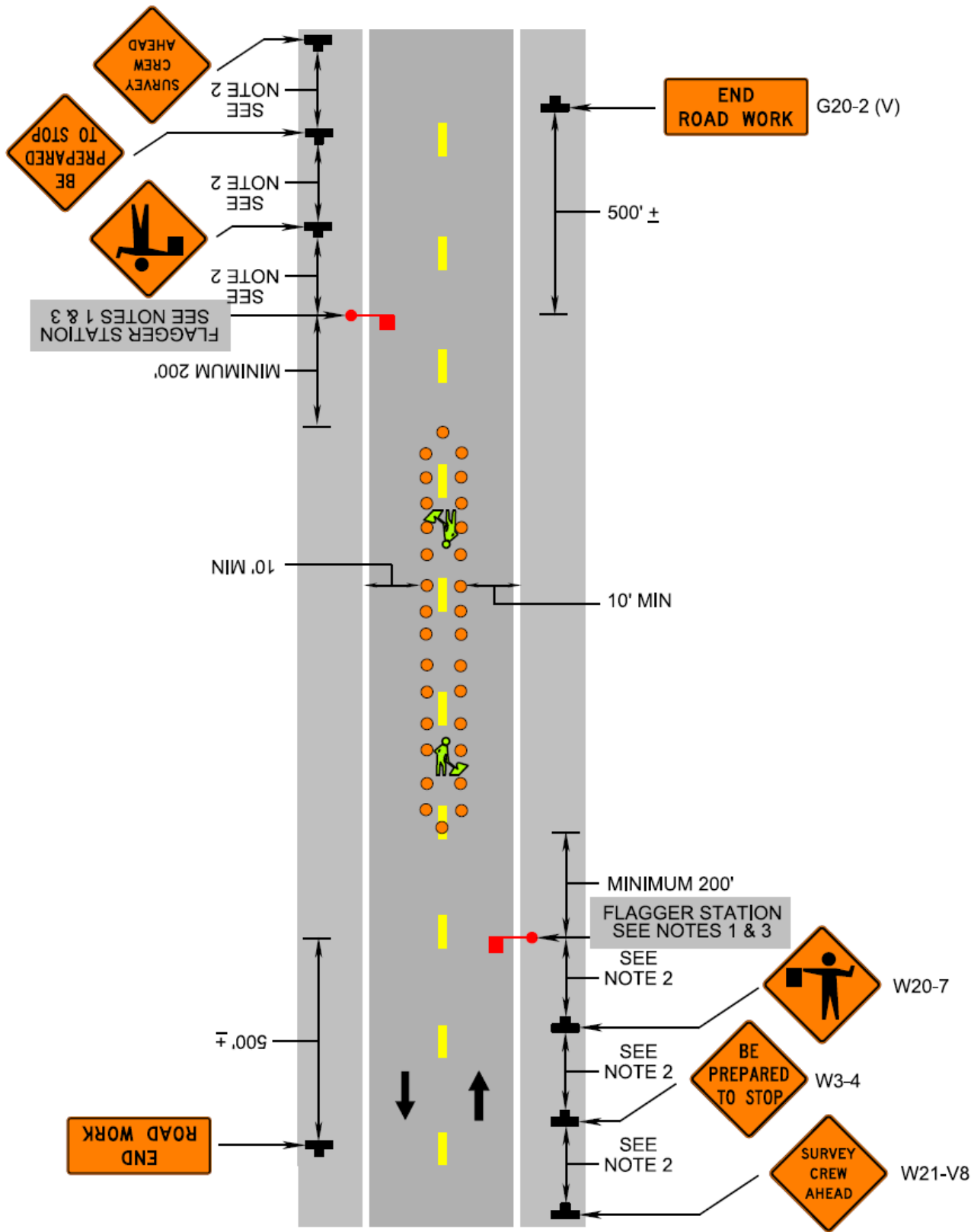
Motorist Survey Operation on a Two-Lane Roadway (Figure TTC-54.1)
