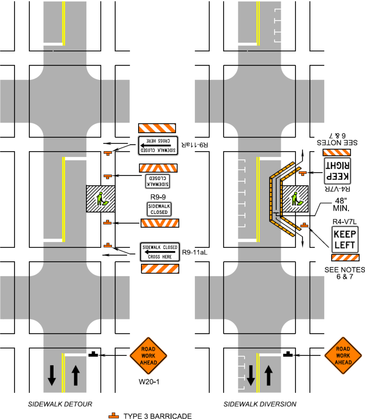
Sidewalk Closure and Bypass Sidewalk Operation (Figure TTC-35.1)
