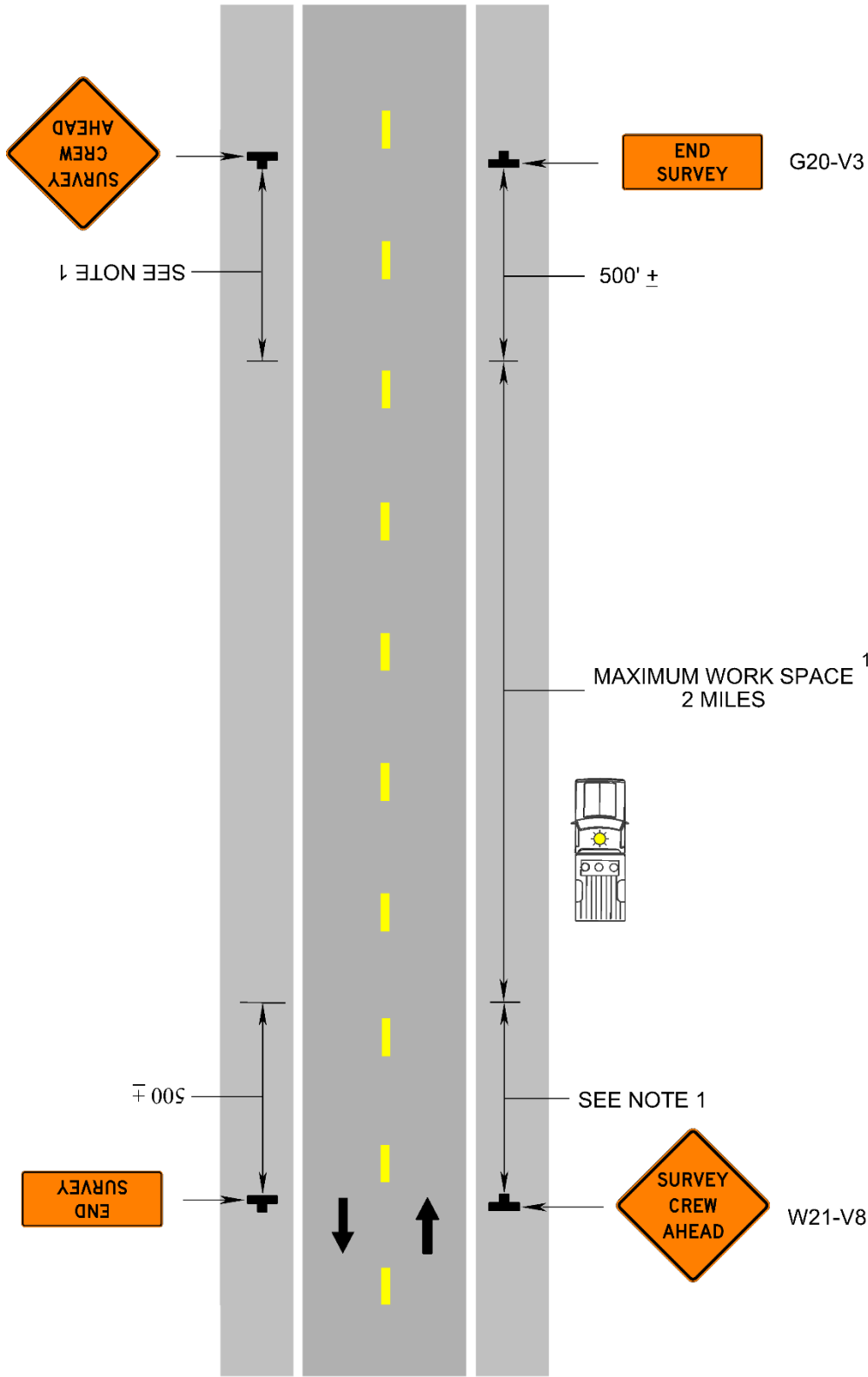
Surveying Operation (Figure TTC-49.1)
