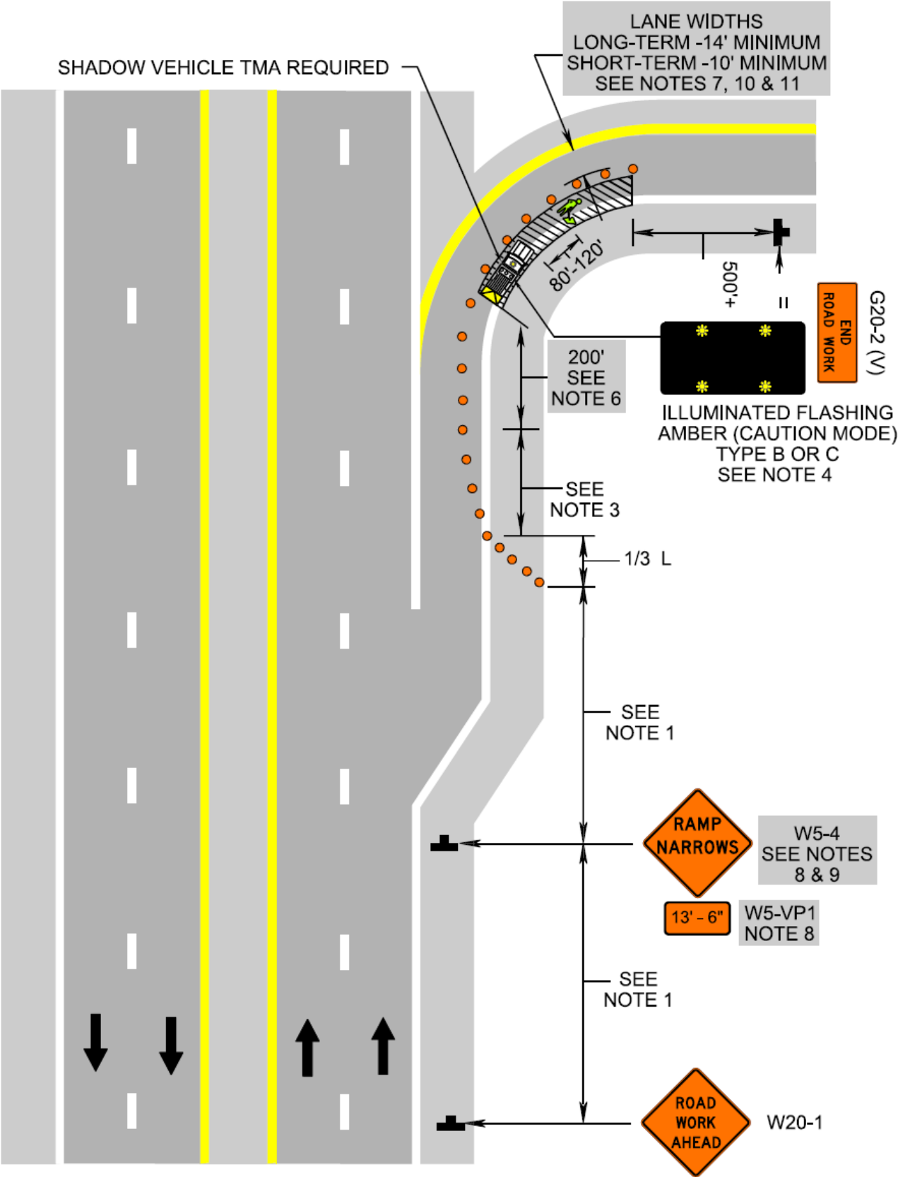
Partial Exit Ramp Closure Operation (Figure TTC-38.2)
