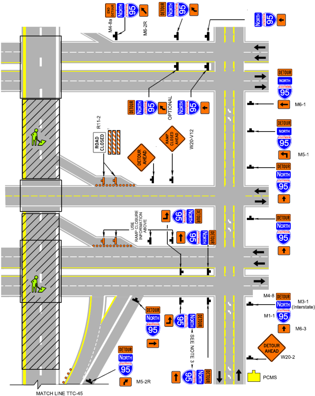
Limited Access Highway Closure Operation with a Long-Term Detour (Figure TTC-47.2)
