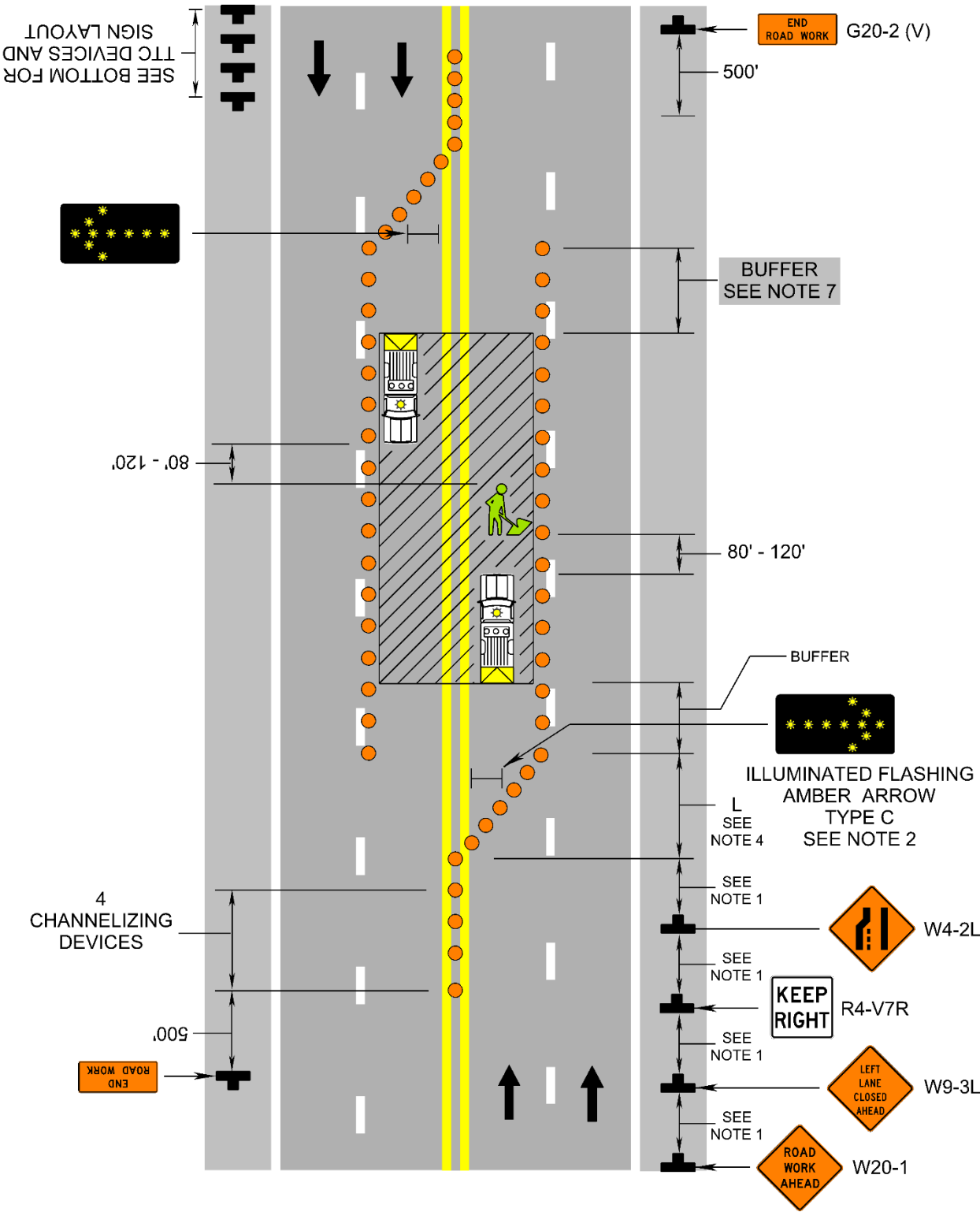
Interior Lane Closure Operation on a Multi-Lane Roadway (Figure TTC-42.2)
