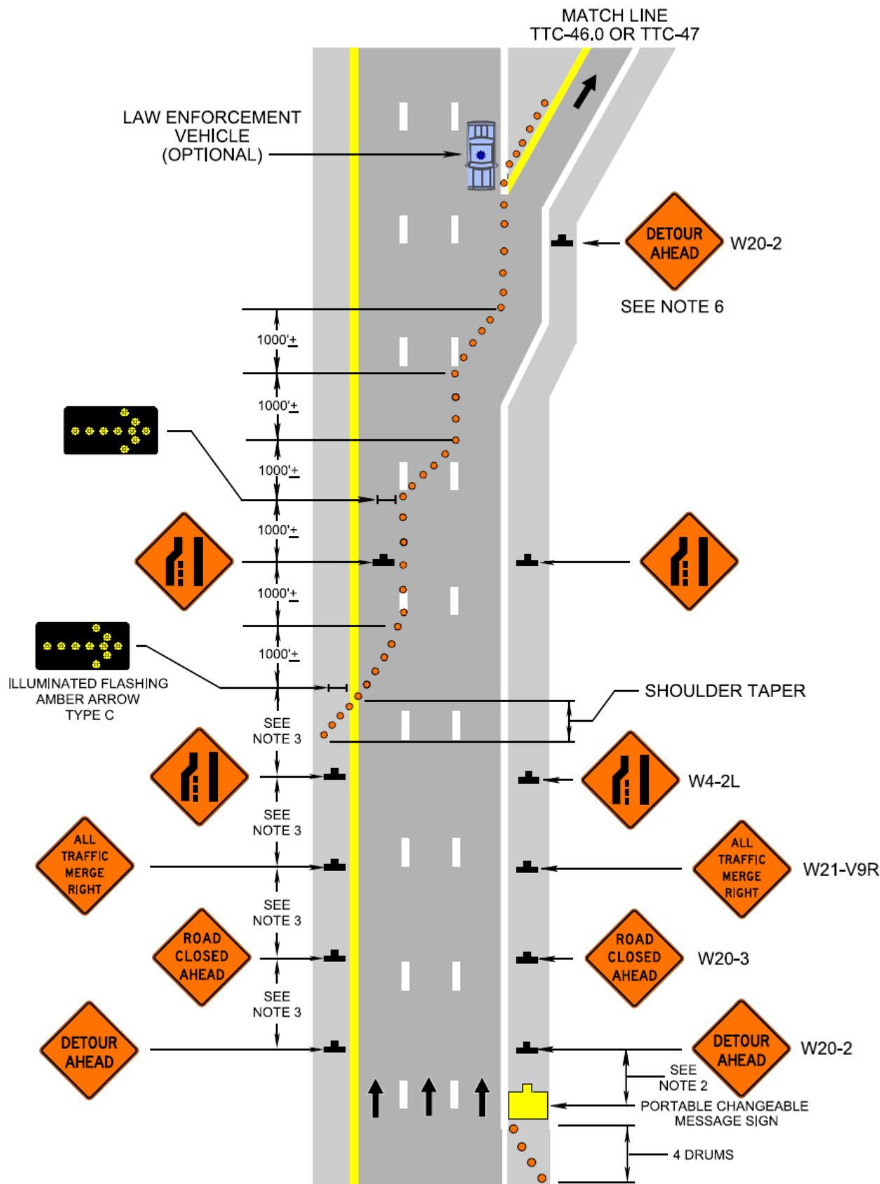
Total Limited Access Highway Closure Operation (Figure TTC-45.2)
