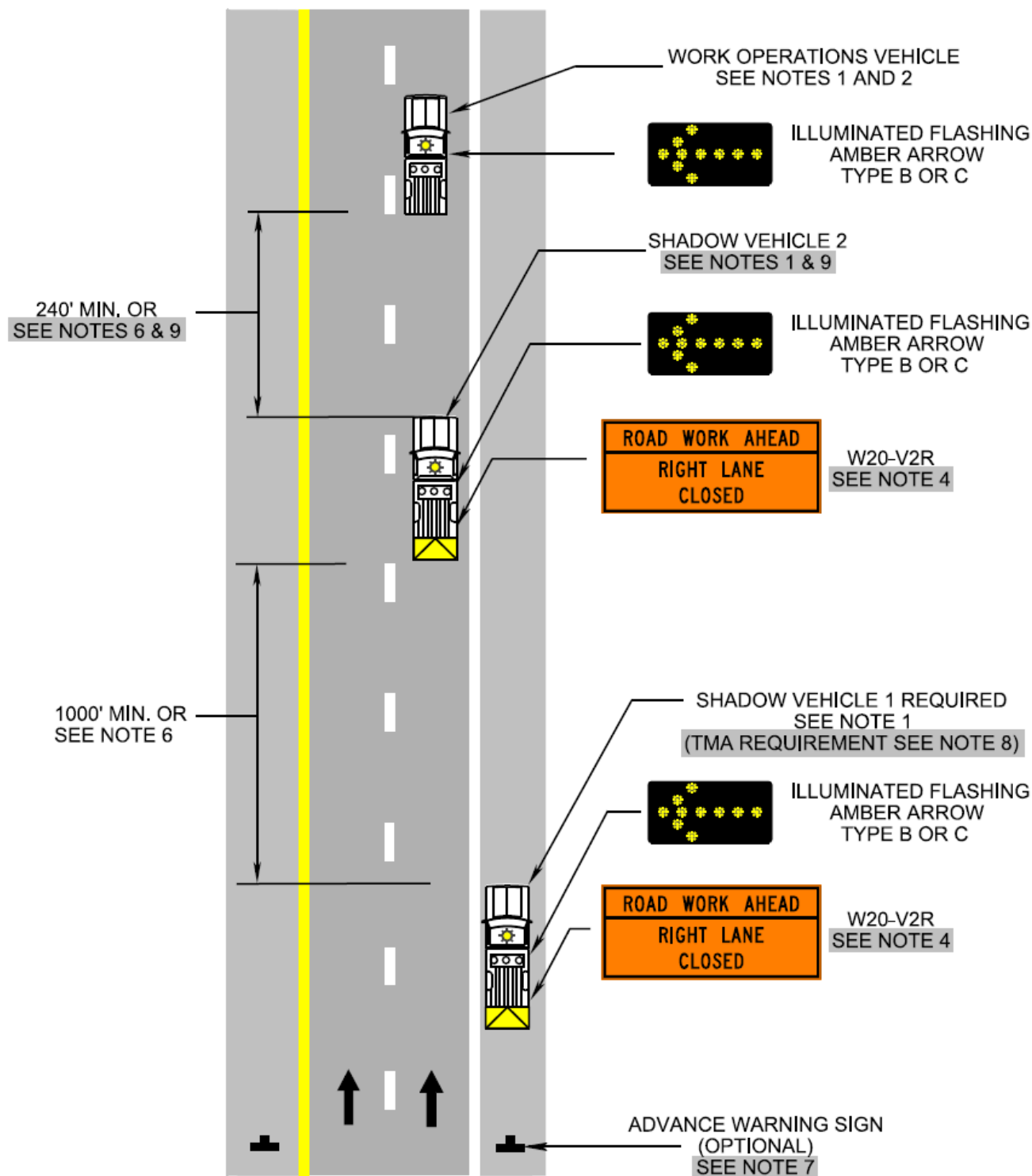
Moving/Mobile Operations on a Multi-Lane Roadway (Figure TTC-13.2)
