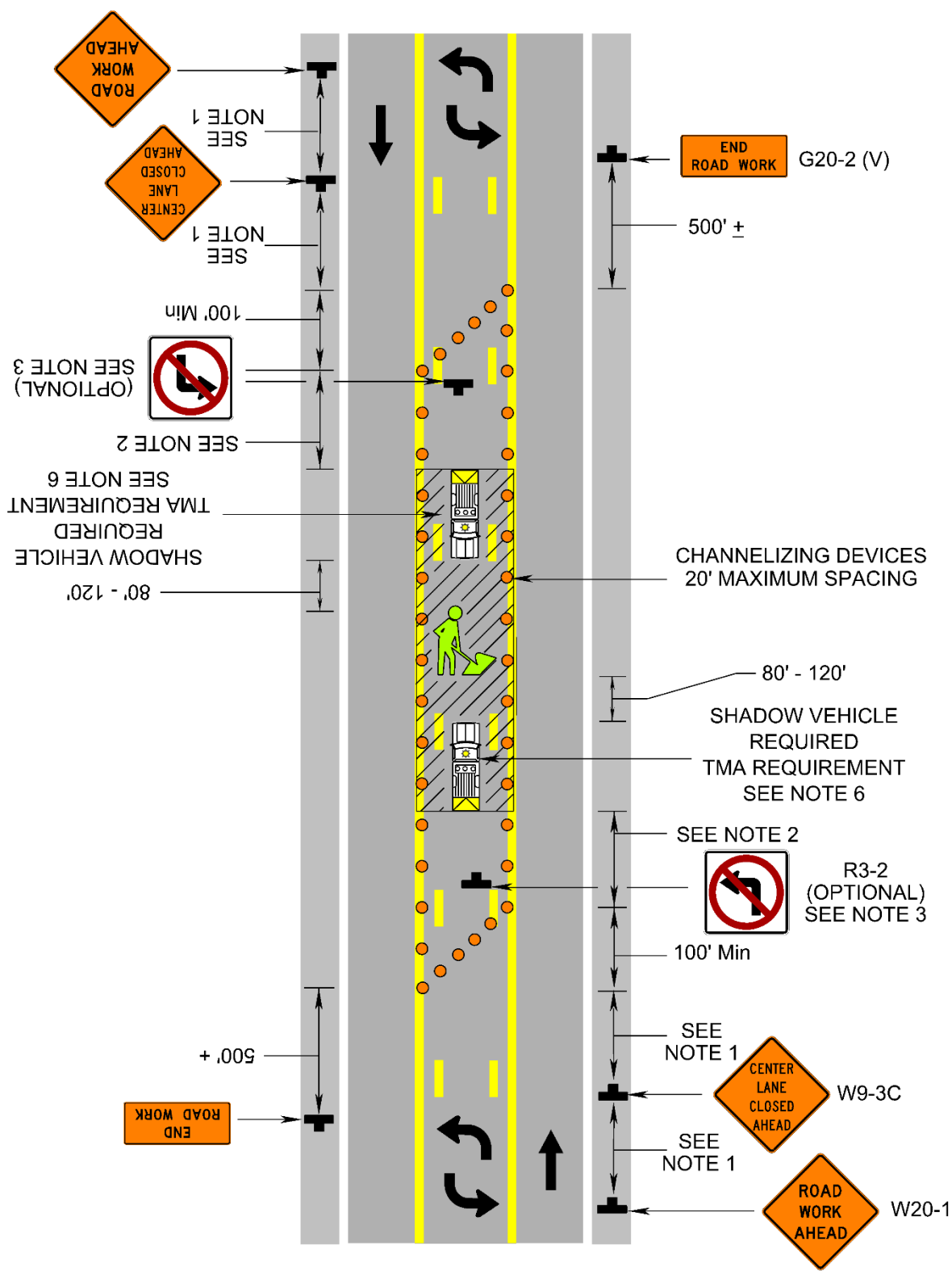
Center Turn Lane Closure Operation (Figure TTC-21.1)
