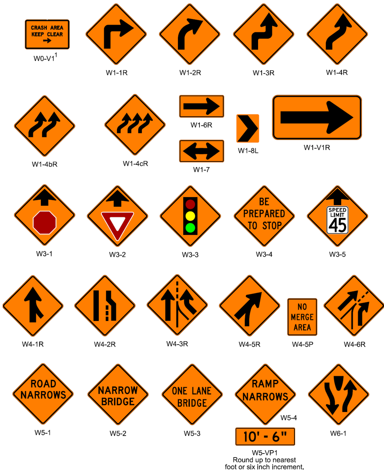
Figure 6F-3, Warning Signs and Plaques in Temporary Traffic Control (Sheet 1 of 5)
