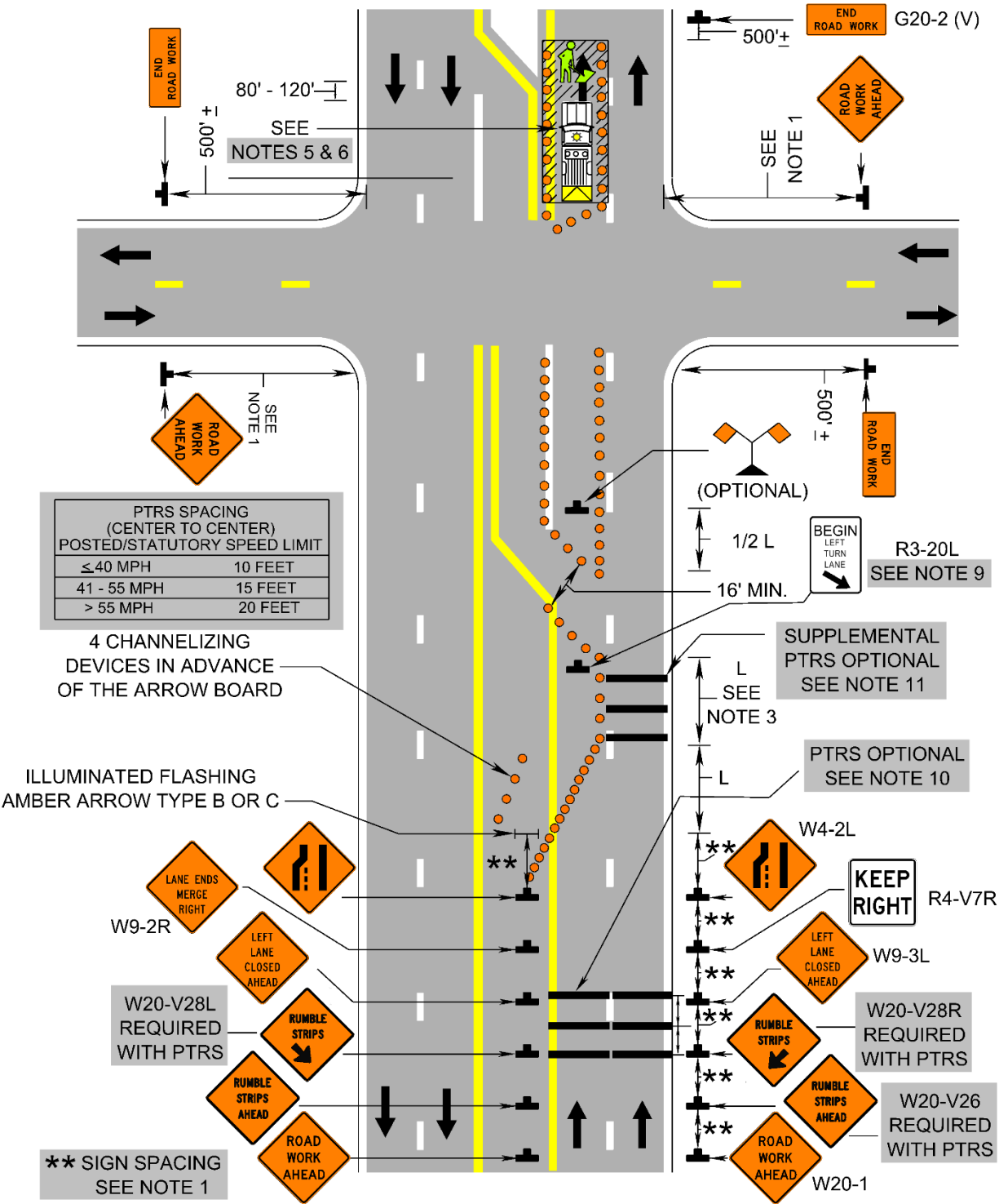
Lane Closure Operation - Far Side of an Intersection (Figure TTC-27.2)
