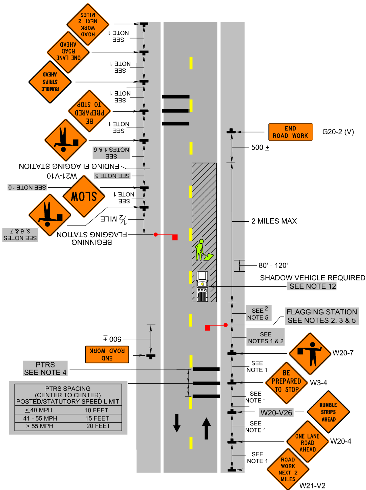
Non-Stationary Operation on a Two-Lane Roadway Using Flaggers (Figure TTC-24.2)
