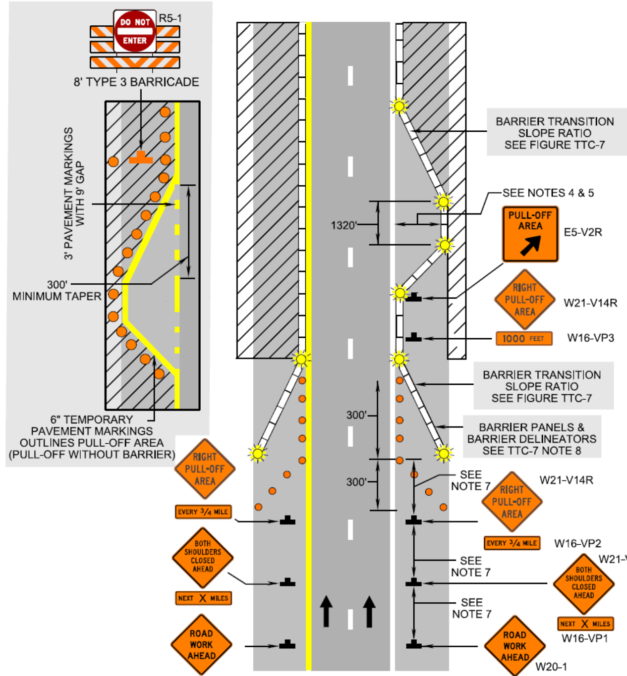
Pull-Off Areas on Limited Access Highways (Figure TTC-8.1)
