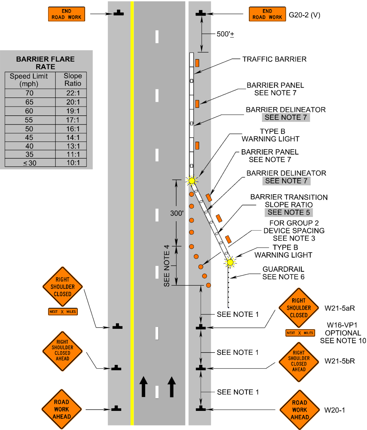
Shoulder Closure with Barrier Operation (Figure TTC-6.2)
