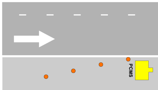
Figure 6F-6, Channelizing Devices for PCMS, Arrow Board and other Trailer Mounted Devices 1
