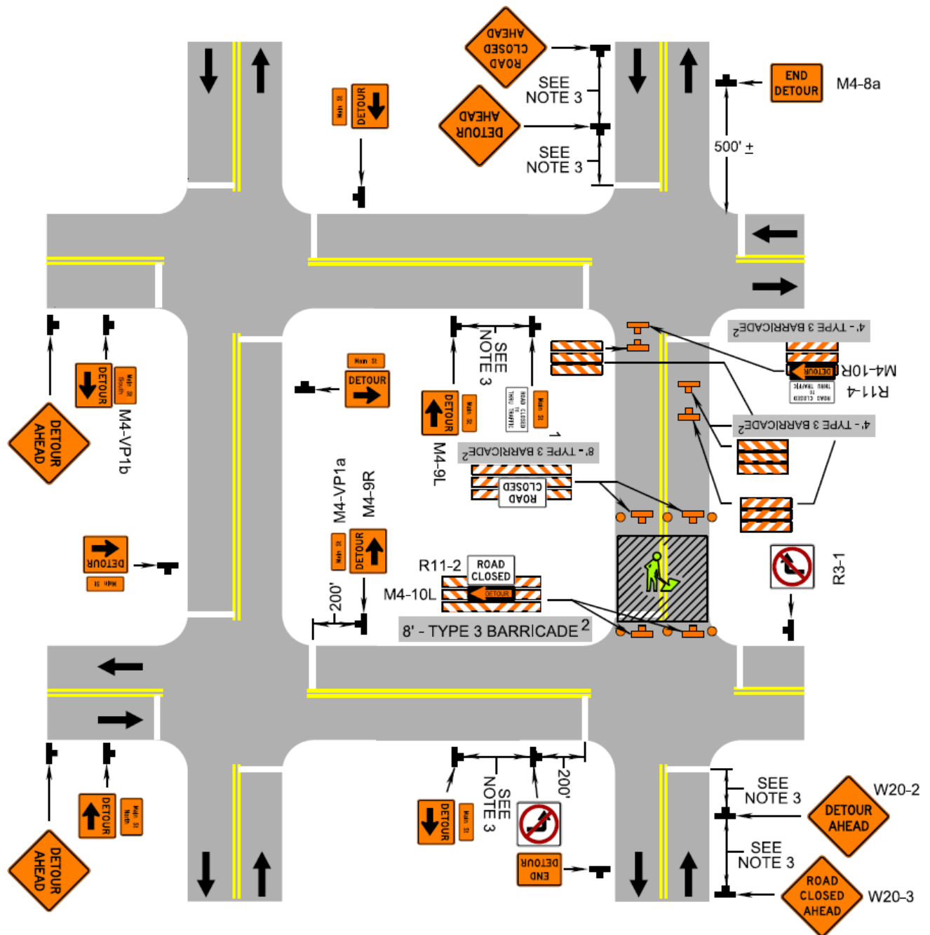
Street Closure Operation with Detour (Figure TTC-34.2)
