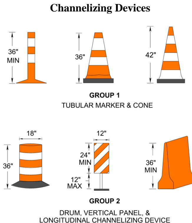
Figure 4, Types of Barriers, and Channelizing Devices
