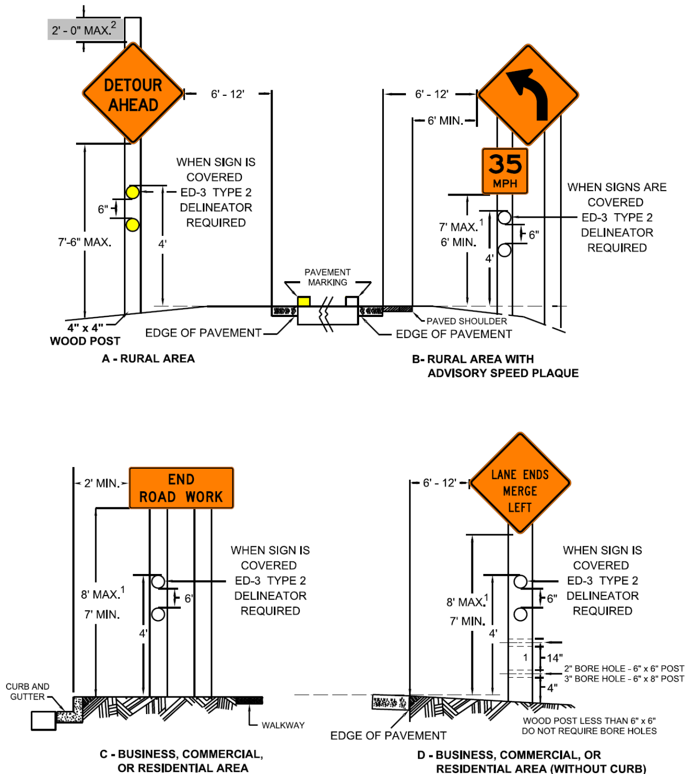
Figure 6F-1, Height and Lateral Location of Signs – Typical Post-Mounted Installations 2
