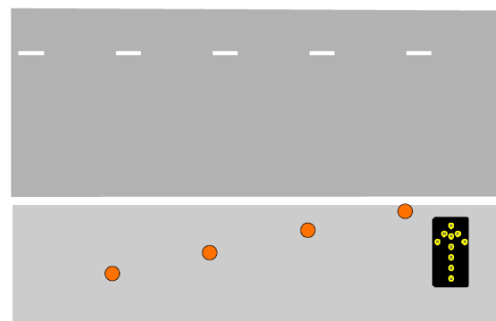
Figure 6F-6, Channelizing Devices for PCMS, Arrow Board and other Trailer Mounted Devices 1
